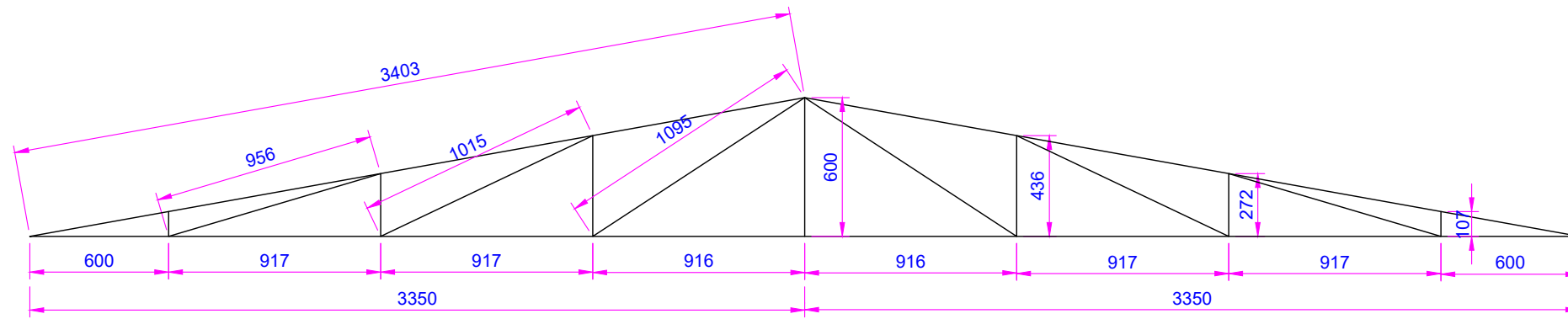
TRUSS ELEVATION
