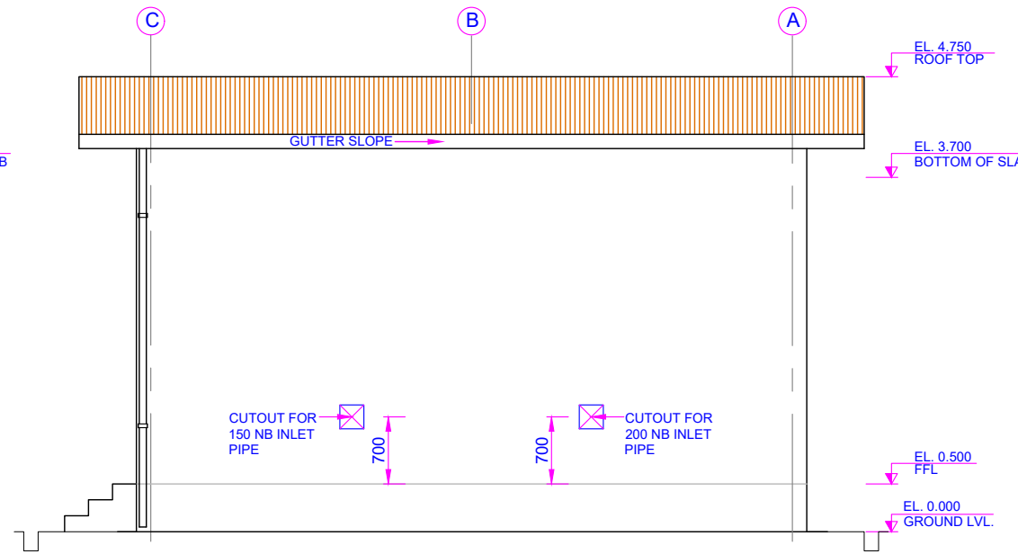
ELEVATION-C
