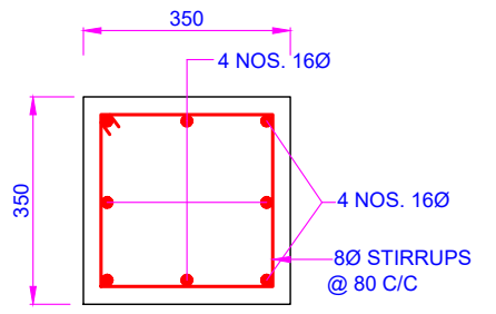
SECTION 3-3
