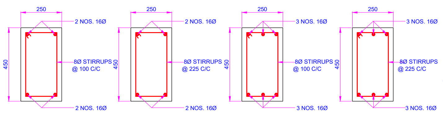
SECTION 1-1
