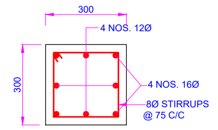
SECTION 1-1
