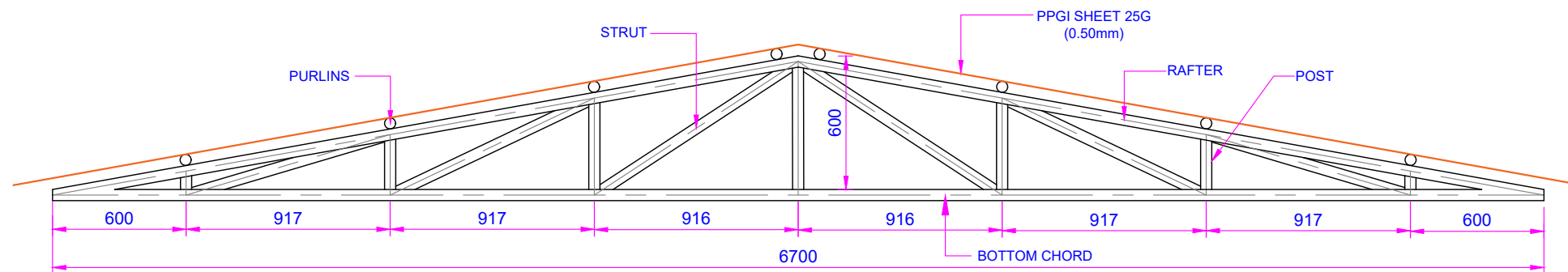
TYPICAL TRUSS DETAILS
