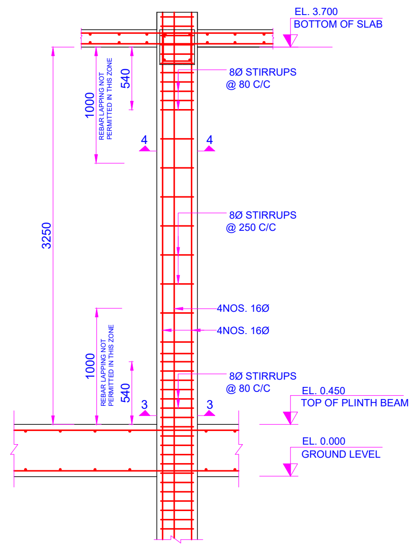
C2 COLUMN DETAILS
