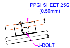
CONNECTION OF PPGI SHEET TO PURLIN & PURLIN TO RAFTER
