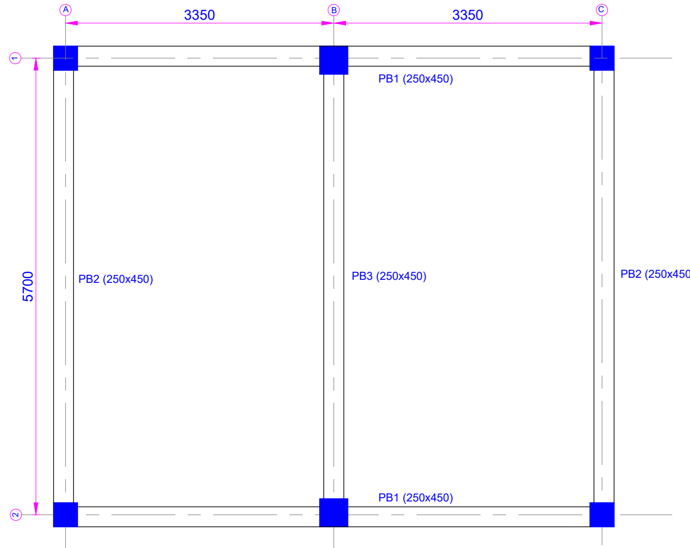
PLINTH BEAM LAYOUT PLAN
