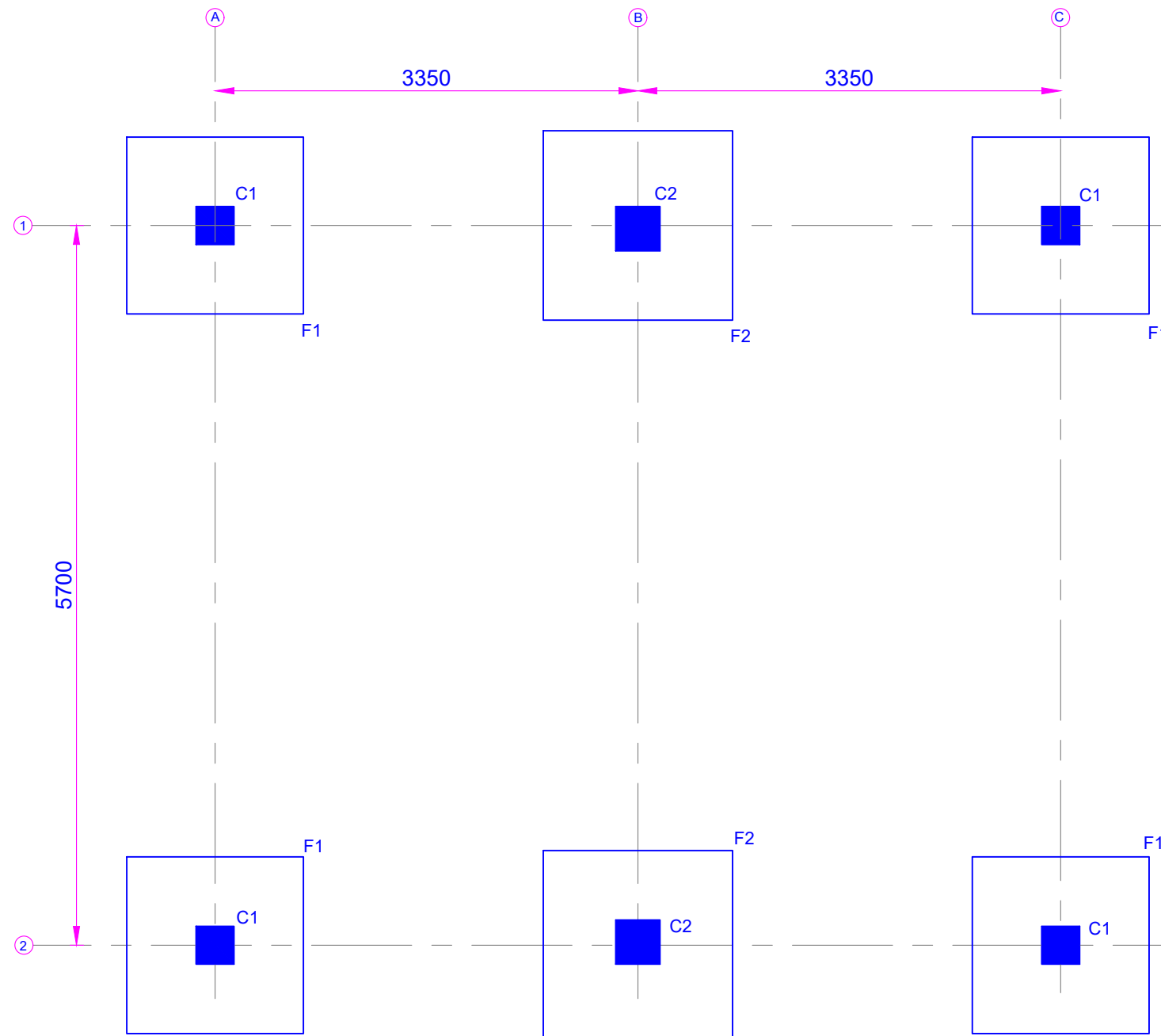
FOOTING LAYOUT PLAN
