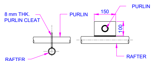
CONNECTION OF PURLIN TO RAFTER
