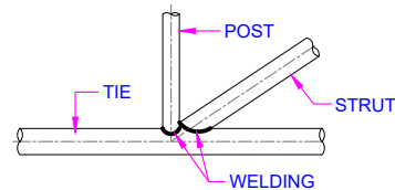
JOINT DETAIL -D
