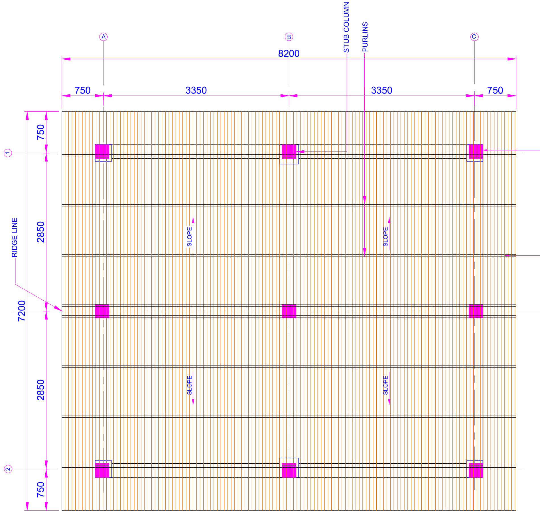
TRUSS LAYOUT PLAN
