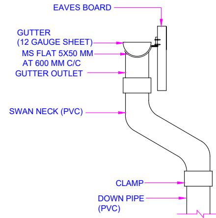
GUTTER DETAILS
