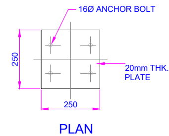
CONNECTION OF TRUSS WITH STUB COLUMN
