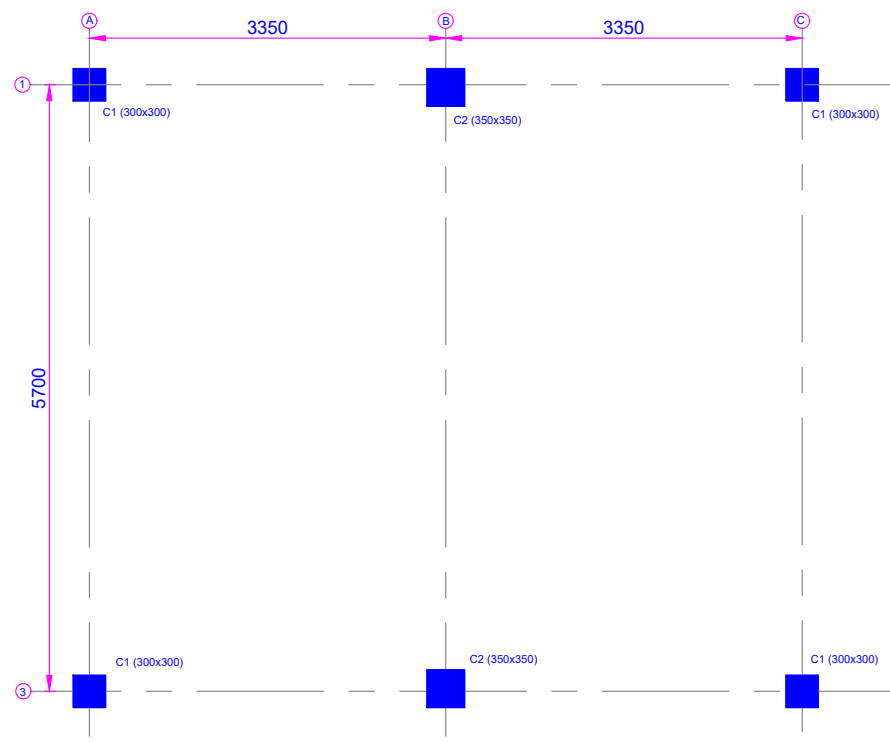
COLUMN LAYOUT PLAN
