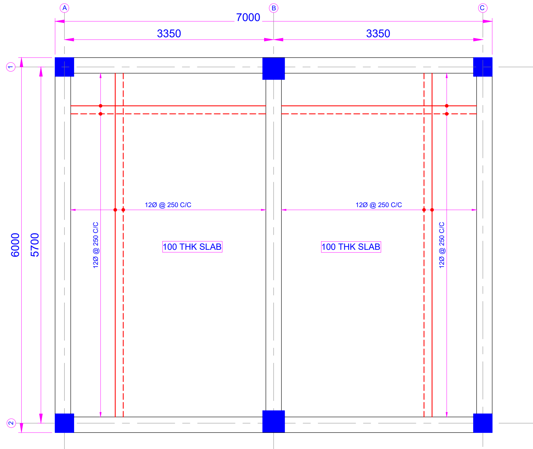
FLOOR SLAB REINFORCEMENT DETAILS
