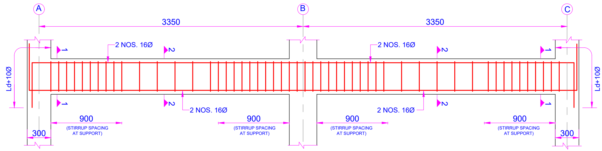
BEAM PB-1
