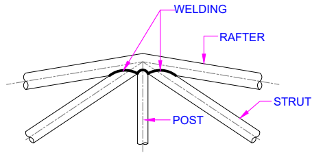
JOINT DETAIL -B
