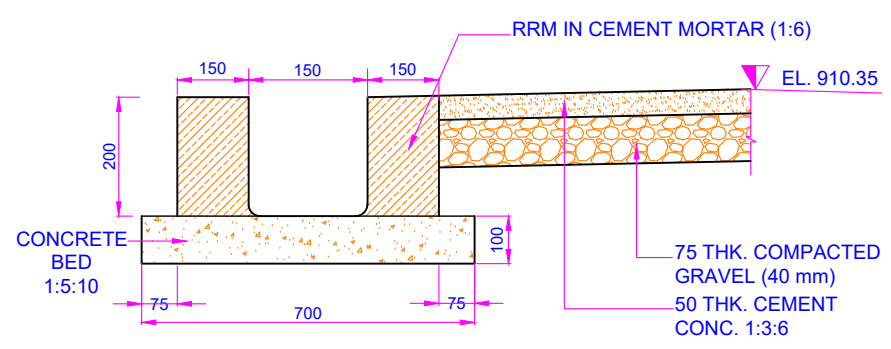
PLINTH PROTECTION & DRAINAGE ARRANGEMENT
