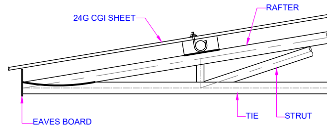
CONNECTION OF CGI SHEET TO PURLIN
