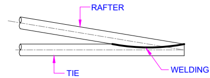
JOINT DETAIL -E
