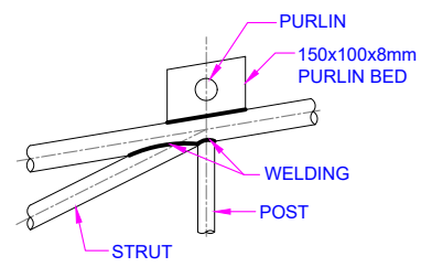
JOINT DETAIL -A
