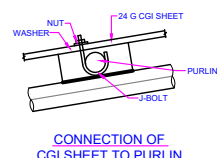
CONNECTION OF CGI SHEET TO PURLIN
