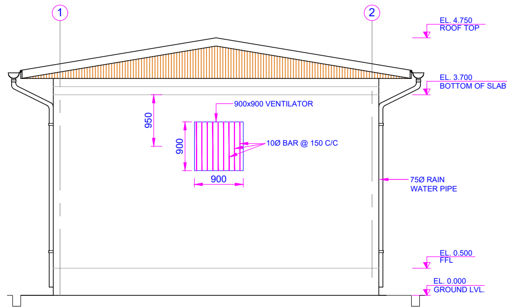
ELEVATION-B
