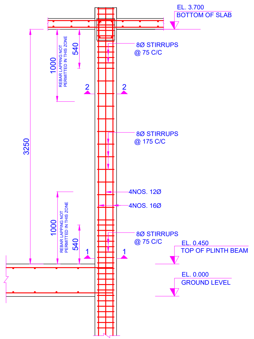
C1 COLUMN DETAILS
